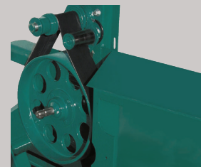
Power band fan speed up system with built-in overrunning clutch
