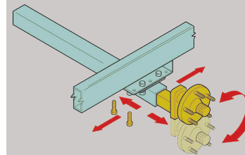
Wheels adjust up or down, in or out, front or rear to obtain best balance and clearance
